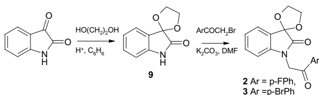
Scheme 2. The synthesis of compounds 2 (1-[(4-fluorophenyl)-2-oxoethyl]-3-(1,3-dioxolano)-2-indolinone) and 3 (1-[2-(4-bromophenyl)-2-oxoethyl]-3-(1,3-dioxolano)-2-indolinone).
