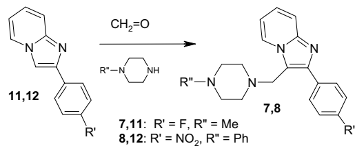
Scheme 4. The synthesis of compounds 6 (3-(morpholinomethyl)-2-(4-fluorophenyl)imidazo[2,1- b ][1,3]thiazole), 7 (2-(4-fluorophenyl)-3-(4-methylpiperazinomethyl)imidazo[1,2- a ]pyridine) and 8 (2-(4-nitrophenyl)-3-(4-phenylpiperazinomethyl)imidazo[1,2- a ]pyridine).
